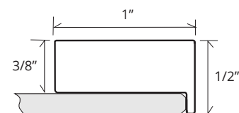
Section view - LEXINGTON FRAME
